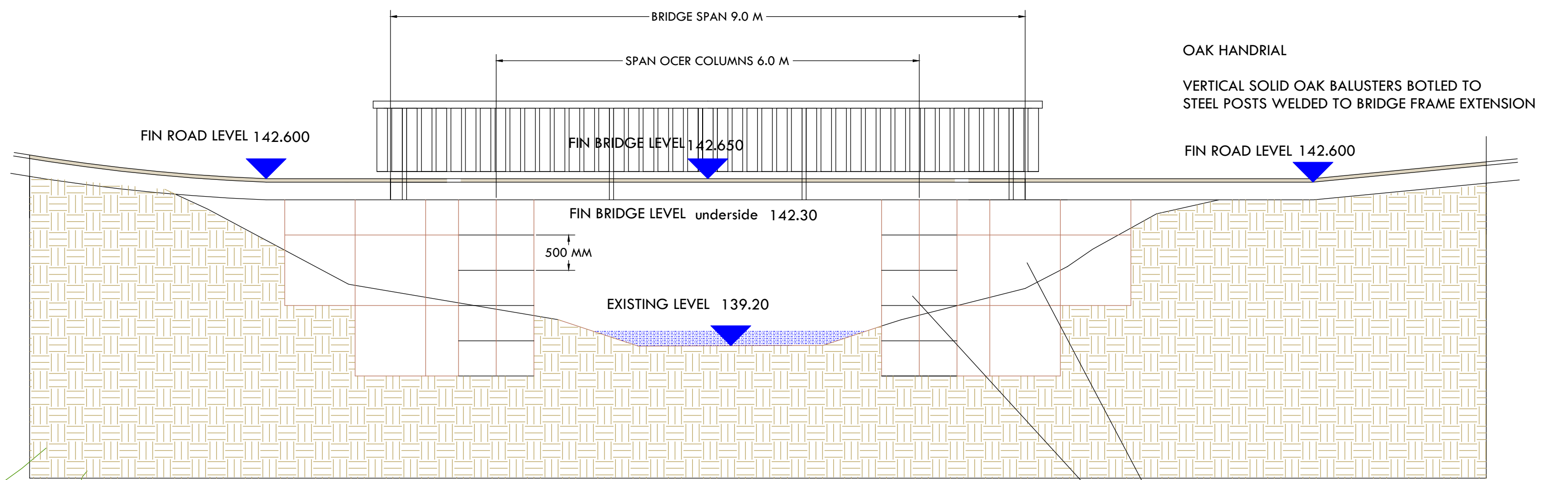
PROPOSED ELEVATION OF BRIDGE 1-50
